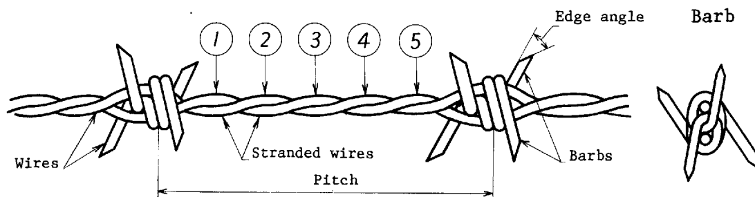
Fig. 1. Iowa type barbed wire
