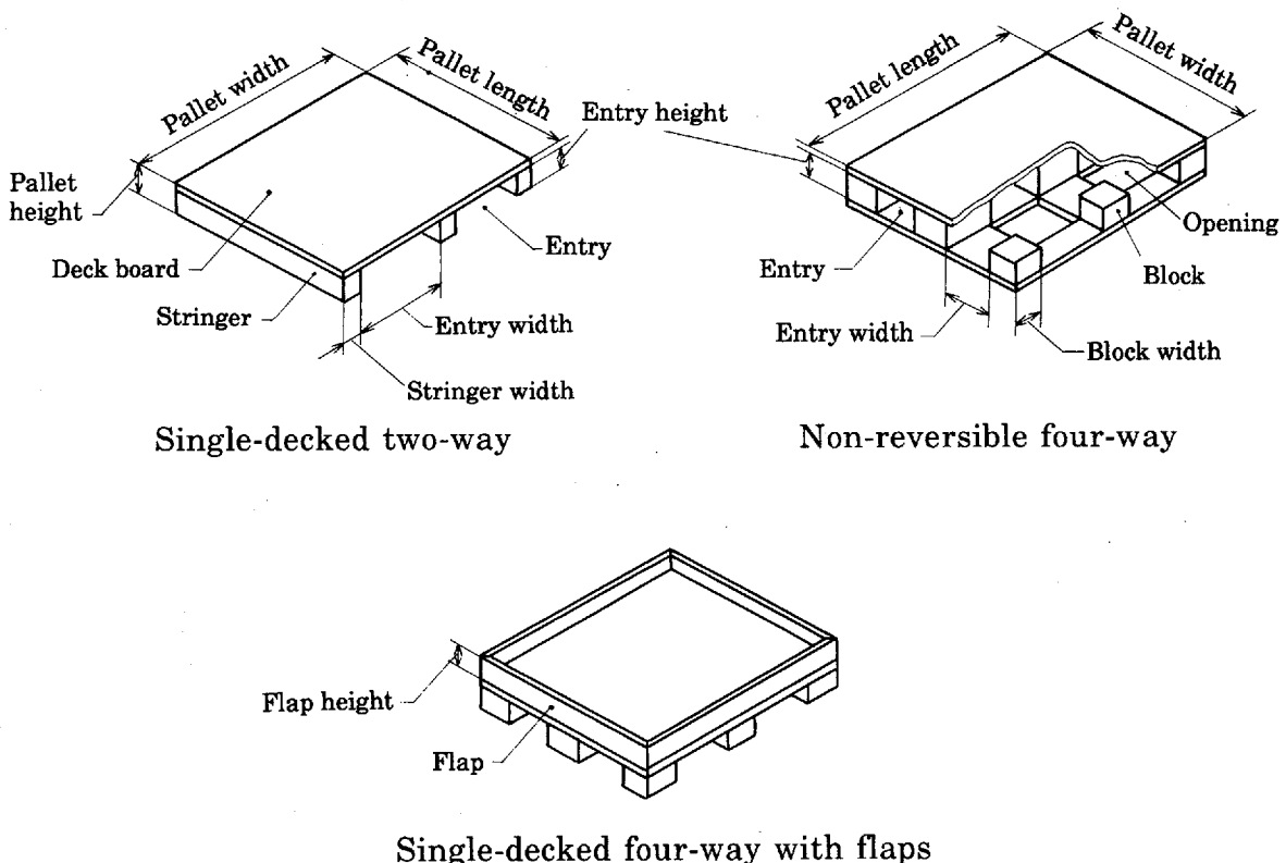
Fig. 1 Name of each part
